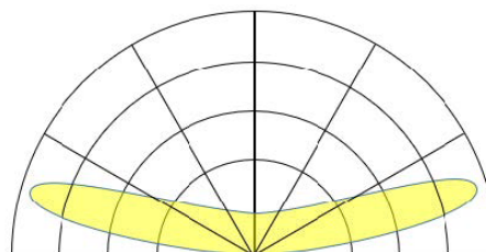
175° Beam Pattern
