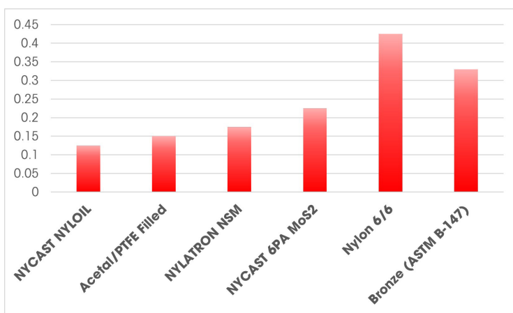
Chart 1: Comparison coefficient of friction on different materials, measured on a thrust washer testing machine, unlubricated at 40 fpm and 50 lb/in 2
